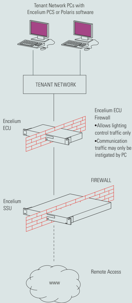
Typical networking connections to enable PCS lighting control. ■
